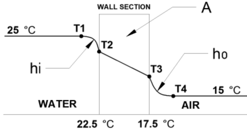
Figure 17: Heat flow through a wall
