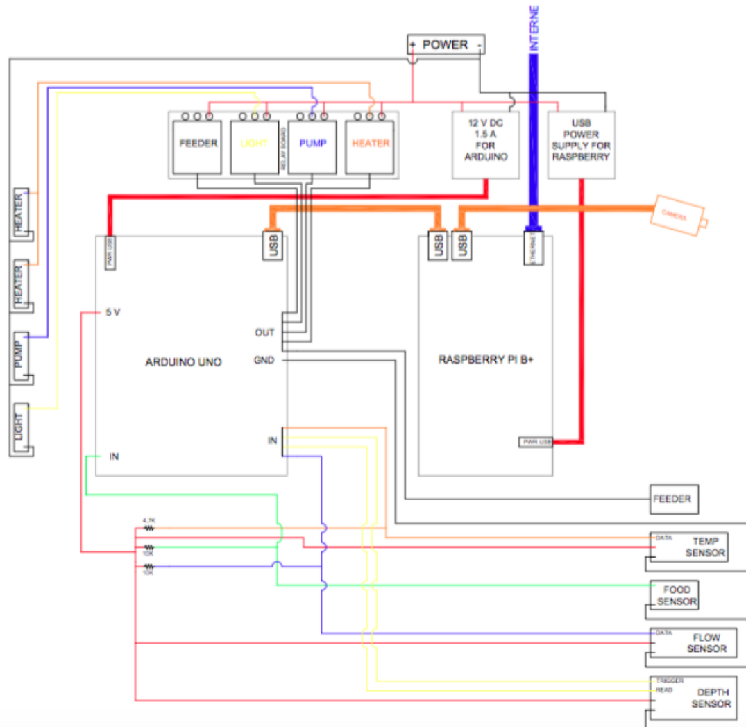
Figure 15: Schematic 1
