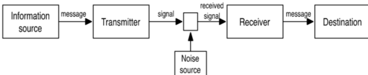
Figure 2: Shannon-Weaver Model
