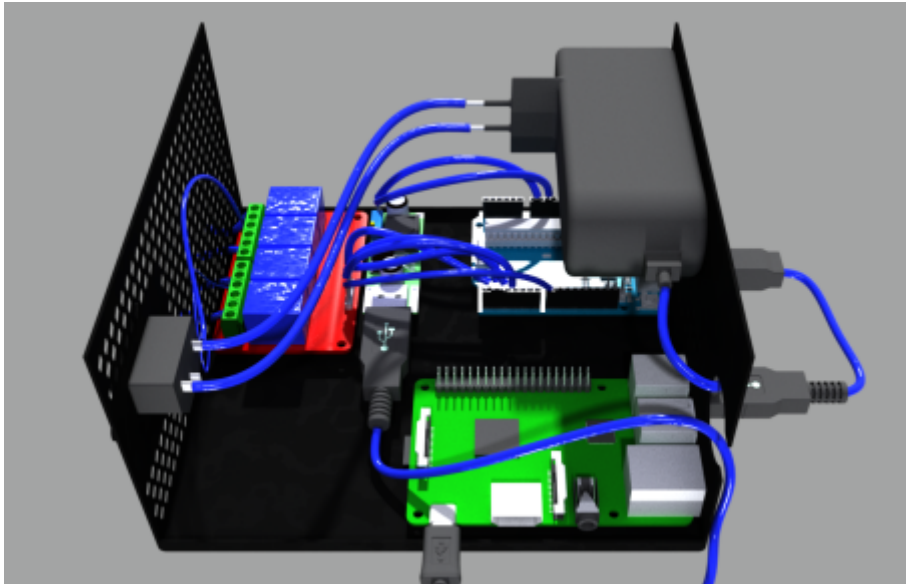
Figure 20: Installed Hardware Components
